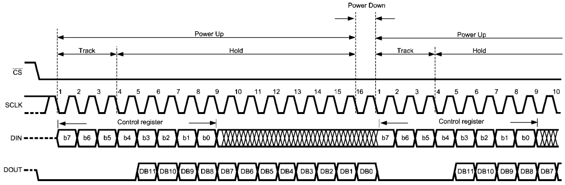
ADC122S051 Operational Timing Diagram
